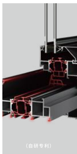
Cold-hot Compression Barrier-Type Insulating Strip (自研专利)
